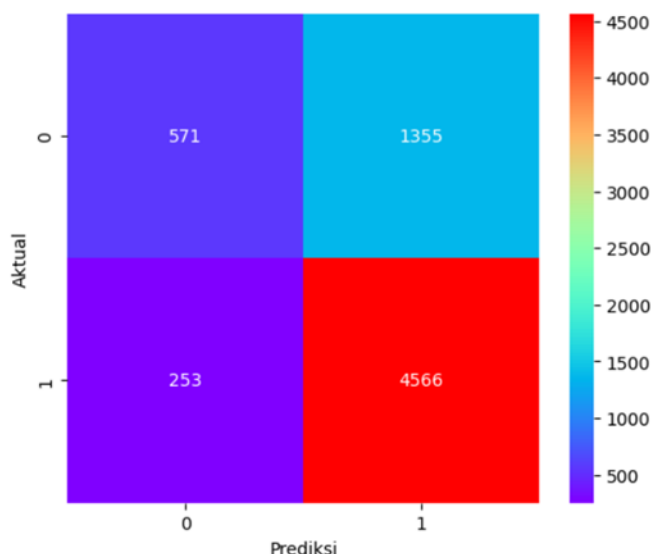
Gambar 2. Confusion Matrix
